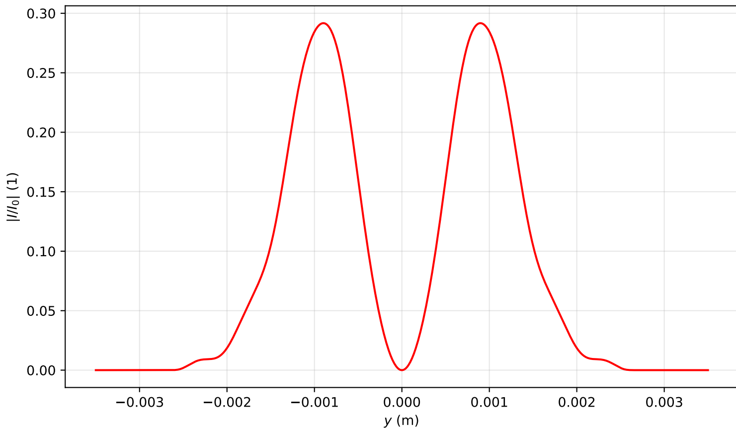
Intensity profile I(x=0, y, z=3.503)/I_0 , \text{Pin}=2.0\text{Pcr} , artificial time
